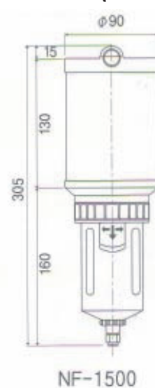
NF-1500 (64 scfm)
