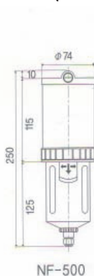
NF-500 (22 scfm)
