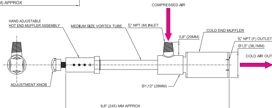
MEDIUM VORTEX TUBE WITH GENERATOR, HAND ADJUSTABLE HOT END MUFFLER ASSEMBLY + COLD MUFFLER
