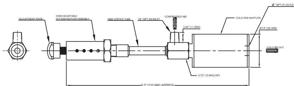
SMALL VORTEX TUBE WITH GENERATOR, HAND ADJUSTABLE HOT END MUFFLER ASSEMBLY + COLD MUFFLER
