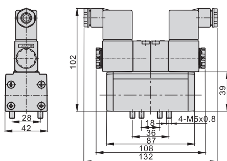
ISO 1 5/2 BCC
